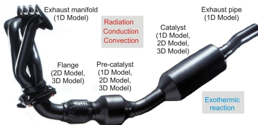
Figure 1. The appearance of the engine exhaust system
