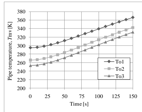
Figure 6. Change in external pipe temperature in pipes 1 before the pre-catalyst
