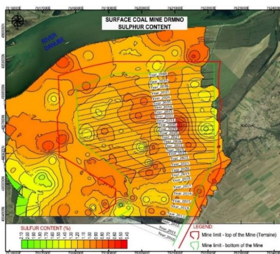
Figure 4. Modelled sulfur content and detailed mine plan
