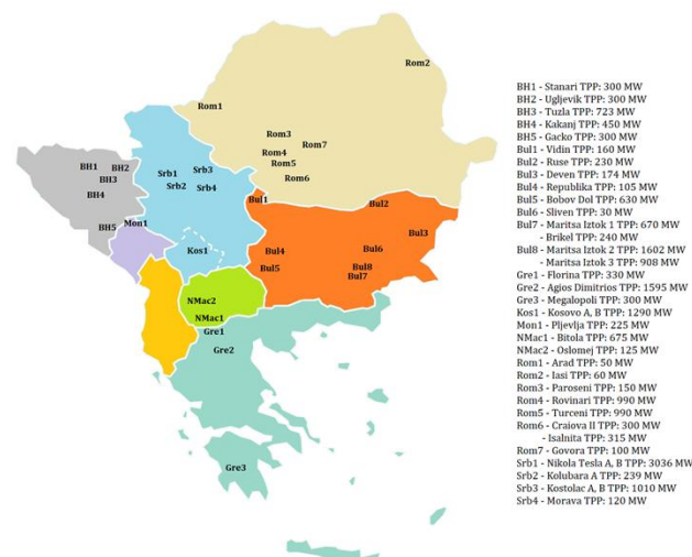
Figure 1. Region SEE with TPP locations
