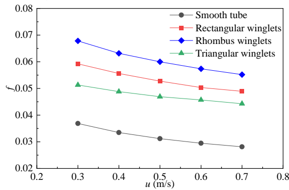
Figure 10. Friction factor of enhanced tube
