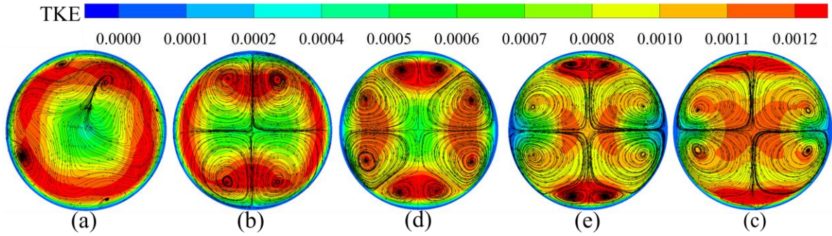
Figure. 13. Effect of five inclination angles of triangular winglets on the flow field structure: (a) \alpha = 0^\circ ; (b) \alpha = 15^\circ ; (c) \alpha = 30^\circ ; (d) \alpha = 45^\circ ; (e) \alpha = 60^\circ
