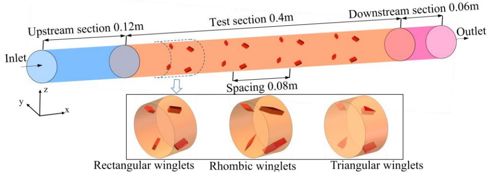
Figure 2. Fluid domain model
