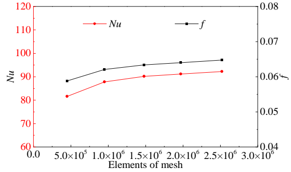
Figure 4. Mesh independence verification
