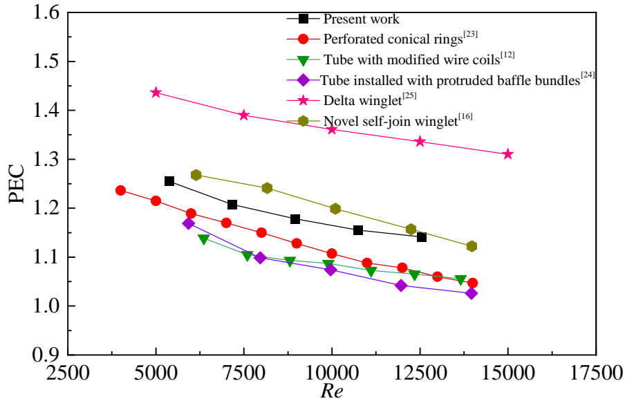
Figure 16. Comparisons of PEC between present work and previous works
