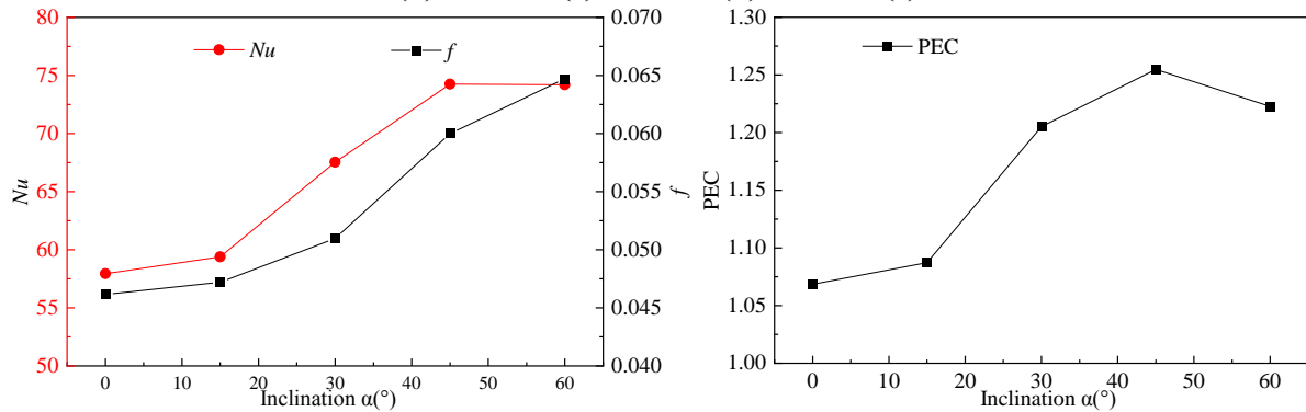
Figure. 14. Variations of Nu and f
