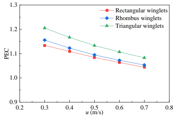
Figure 12. PEC of enhanced tube
