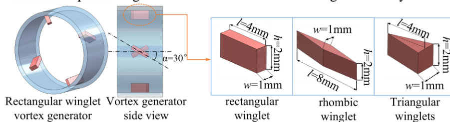
Figure 1. Three types of winglet vortex generator
