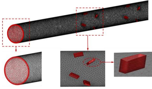
Figure 3. Fluid domain mesh
