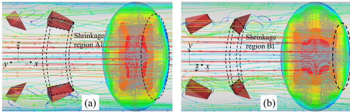
Figure 7. Two shrinkage regions: (a) shrinkage region A1; (b) shrinkage region B1
