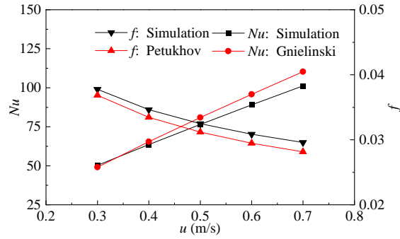
Figure 5. Numerical method validation
