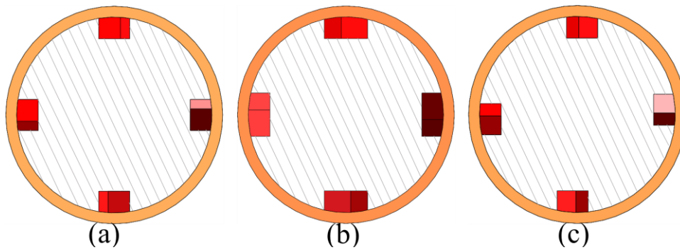
Figure 11. Blockage area: (a) rectangular winglets; (b) rhombic winglets; (c) triangular winglets
