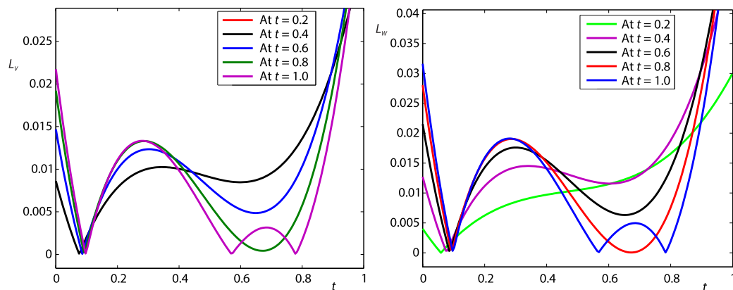
Figure 4. Absolute errors in v and w at different values of t for variable order \theta = 1 - \exp(-t) and scale Level 6 of Example 1
