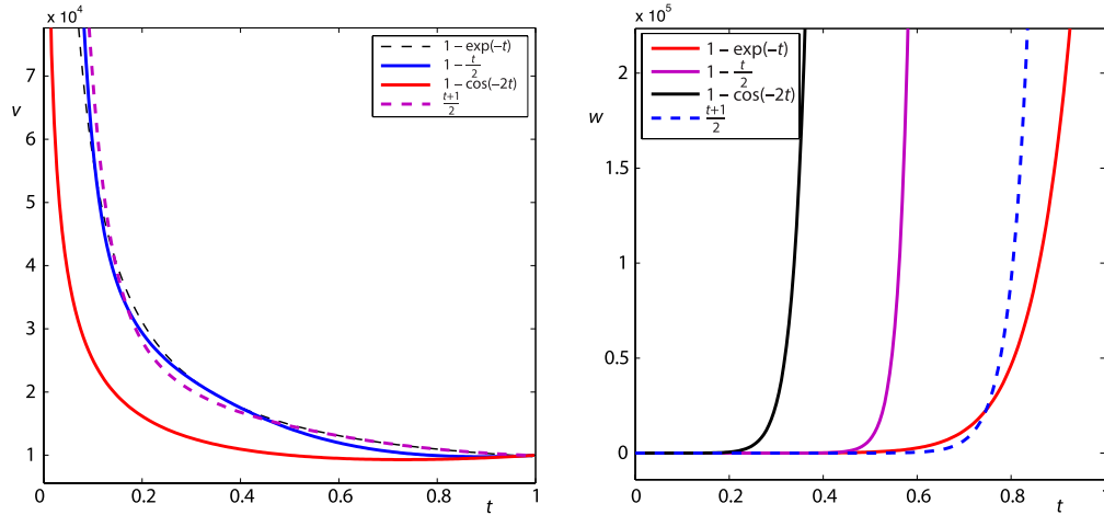
Figure 7. Graphical presentation of numerical solutions of v and w at scale Level 6 and different variable orders of Example 2
