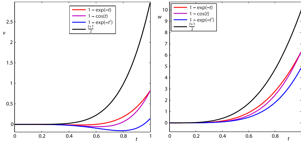
Figure 11. Graphical presentation of numerical solutions of v and w at scale Level 6 and different variable orders of Example 3
