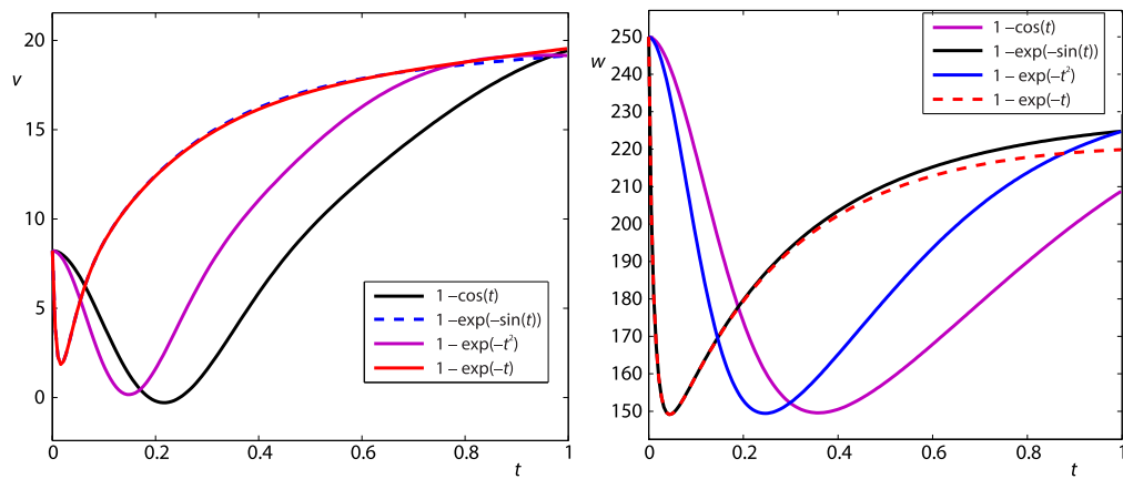
Figure 3. Graphical presentation of numerical solutions of v and w at scale Level 6 and different variable orders of Example 1
