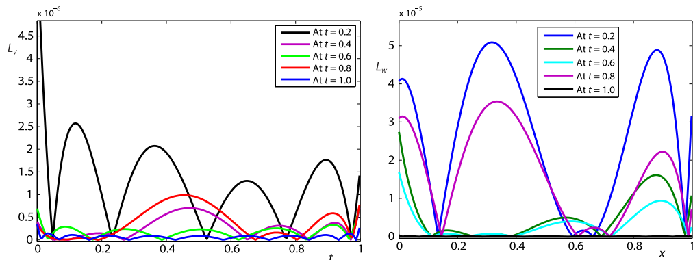
Figure 12. Absolute errors in v and w at different values of t for \theta = (t + 1)/2 and scale Level 6 for Example 3
