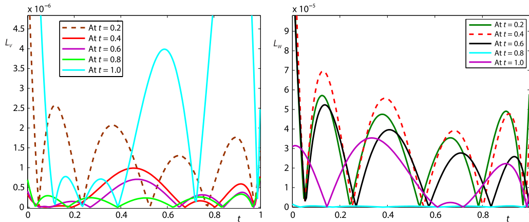
Figure 8. Absolute errors in v and w at different values of t for variable order \theta = 1 - t/2 and scale Level 6 of Example 2
