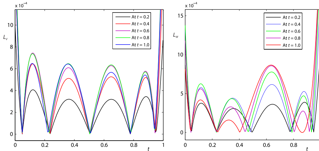
Figure 16. Absolute errors in v and w at different values of t for \theta = 1 - (t/2) and scale Level 6 for Example 4
