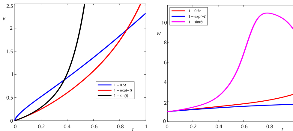
Figure 15. Graphical presentation of numerical results for v and w at different variable fractional order and scale Level 6 for Example 4
