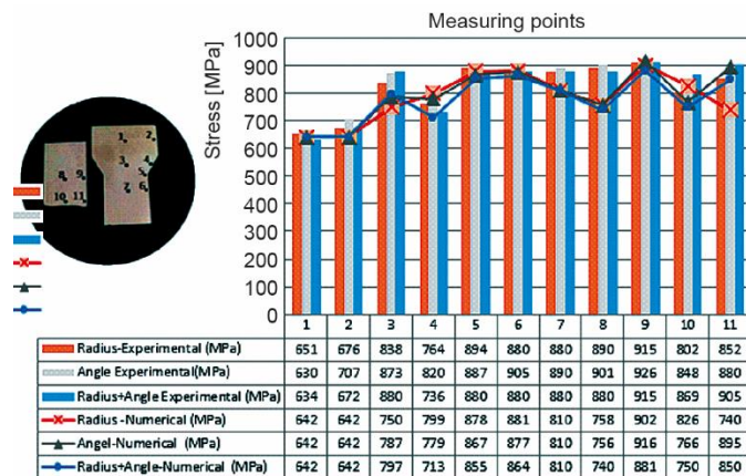
Figure 8. Experimental and numerical examination of the data obtained according to the hardness measurement zones in the radius-angle mold sample
