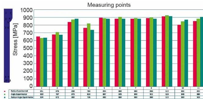
Figure 7. Experimental and numerical analysis of the data obtained according to the hardness measurement zones in the radius-angle mold sample
