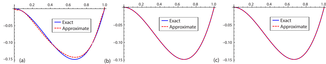
Figure 1. Graphics of exact and approximate solutions for Example 1 when N = 4, 16 , and 64 ; (a) N = 4 , (b) N = 16 , and (c) N = 64
