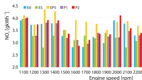
Figure 7. The effect of ethanol on NO x emissions
