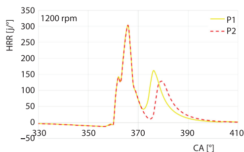
Figure 11. Change of HRR with ethanol post injection at 1200 rpm
