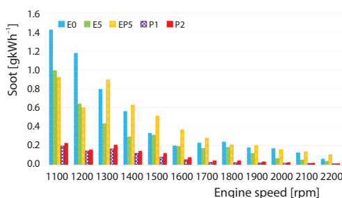
Figure 8. The effect of ethanol on soot emissions
