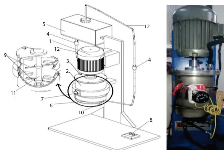
Figure 4. Electric mixer system with temperature control and fuel pump; 1 – AC motor, 2 – mixing chamber, 3 – fuel injection nozzle, 4 – fuel pump, 5 – fuel tank, 6 – heater, 7 – thermostat control, 8 – system control, 9 – blender propeller, 10 – fuel output for main tank, 11 – blender shaft, and 12 – fuel line
