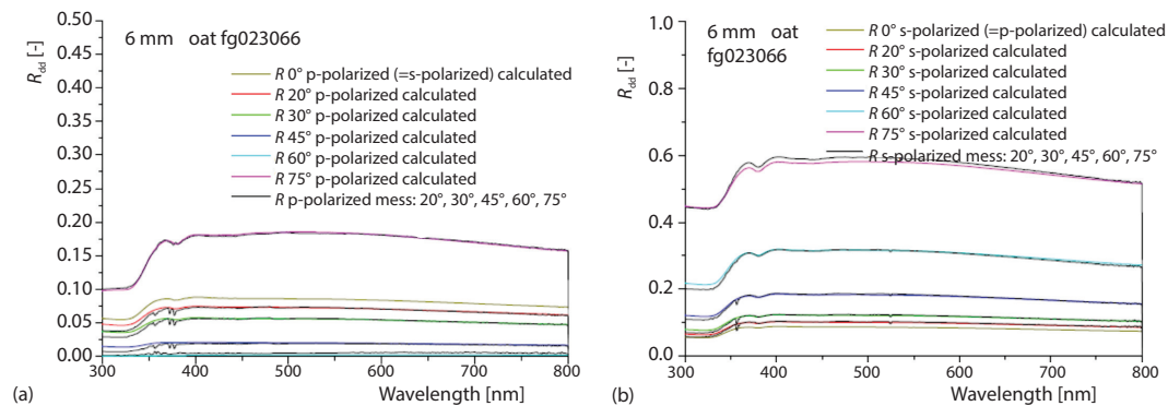
Figure 28. Reflectance spectra of 6mm float glass for p- and s-polarized light and different angles of incidence [21]
