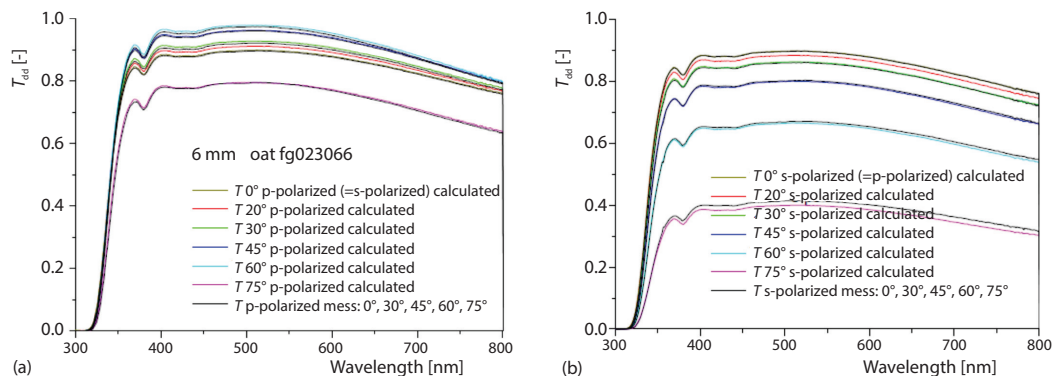
Figure 27. Transmittance spectra of 6 mm float glass for p- and s-polarized light and different angles of incidence [21]
