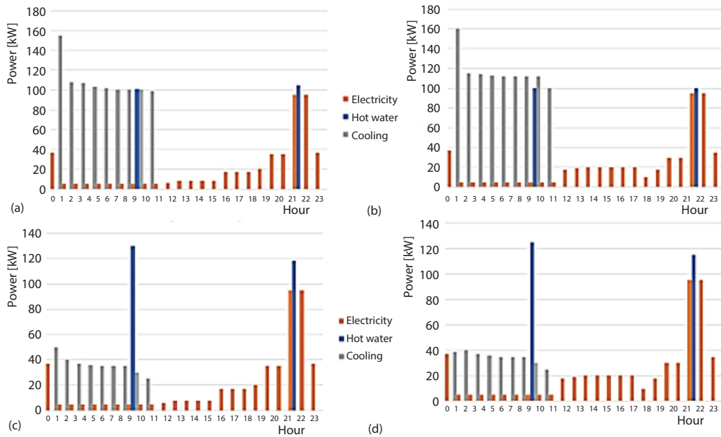
Figure 3. Energy demands for a representative day in January; (a) weekday and (b) weekend and a representative day in August; (c) weekday and (d) weekend
