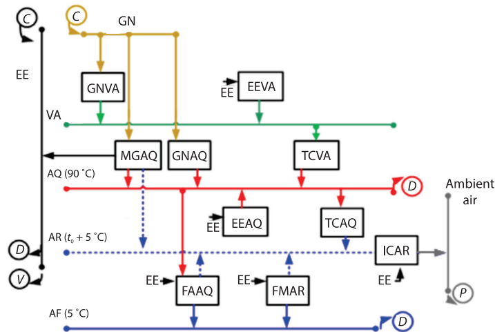
Figure 2. Superstructure of the energy system
