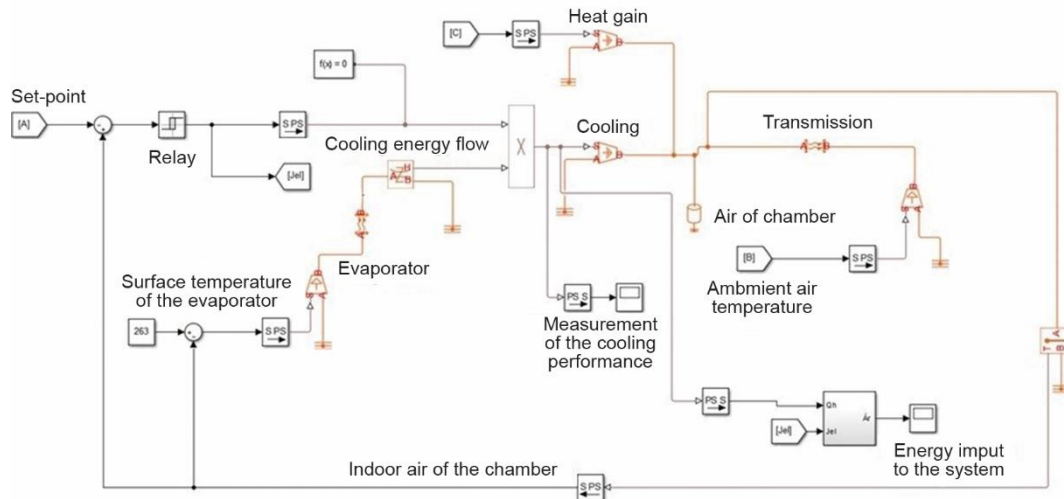
Figure 1. The connection diagram of simulation model for the system with ON/OFF control
