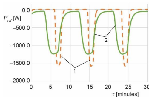
Figure 6. The change of cooling power over time in case of the corrected and the extended simulation; 1 – corrected simulation values, 2 – extended simulation values
