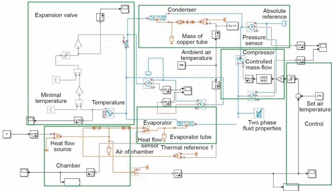
Figure 4. Schematic diagram of the extended simulation model for refrigeration cycle
