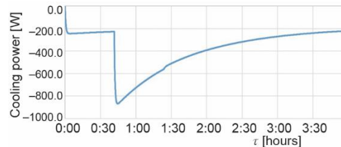
Figure 11. The cooling power fluctuation in the PID controlled chamber over time after placement of the goods
