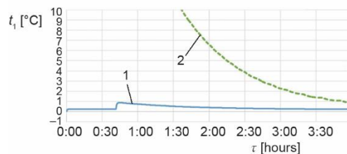
Figure 9. The temperature fluctuation of air in PID controlled chamber and the goods over time; 1 – chamber temperature, 2 – goods temperature
