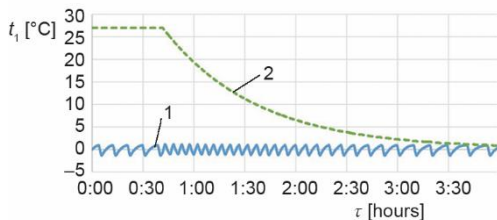
Figure 8. The temperature fluctuation of air in ON/OFF controlled chamber and the goods over time; 1 – chamber temperature, 2 – goods temperature
