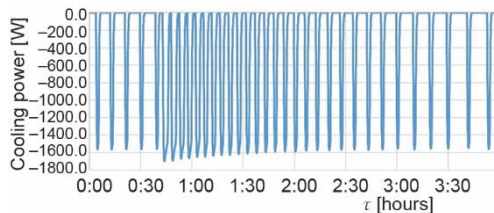
Figure 10. The cooling power fluctuation in the ON/OFF controlled chamber over time after placement of the goods
