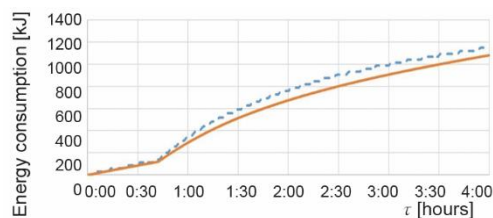
Figure 12. The energy consumption changing of the PID and ON/OFF controlled refrigeration systems over time following the placement of the goods
