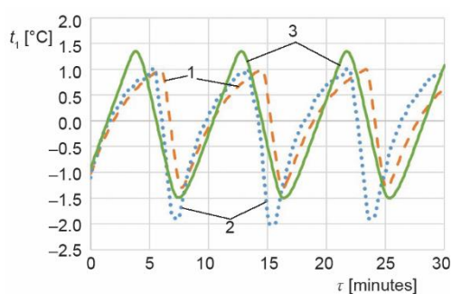
Figure 5. The change of chamber indoor air temperature over time based on measured, corrected simulation and extended simulation calculations in case of refrigeration systems with ON/OFF control; 1 – corrected simulation values, 2 – measured data, 3 – extended simulation values
