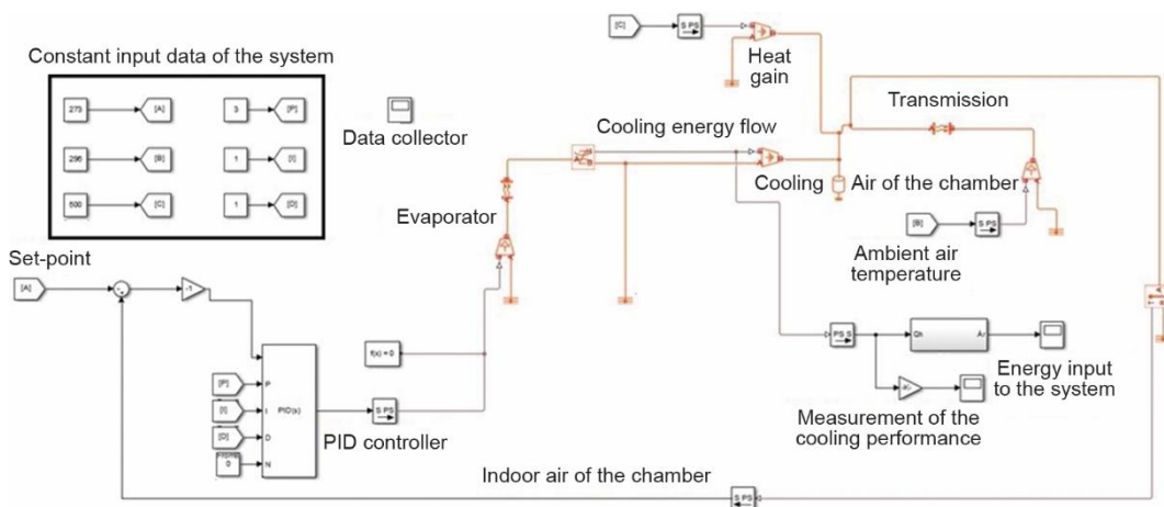
Figure 2. The connection diagram of simulation model for the system with PID control
