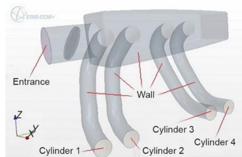
Figure 4. Boundaries and region of the intake manifold CFD model
