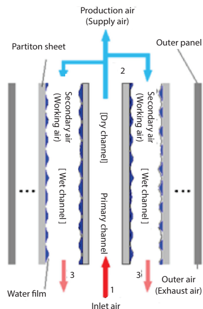
Figure 1. Schematic of counter flow HMX
