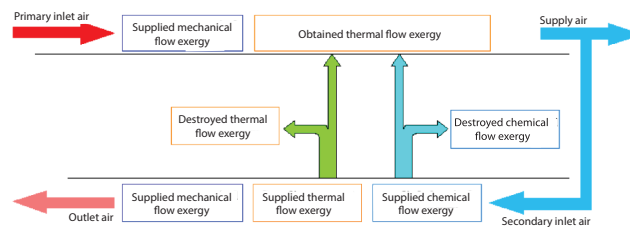
Figure 3. The schematic diagram of exergy analysis
