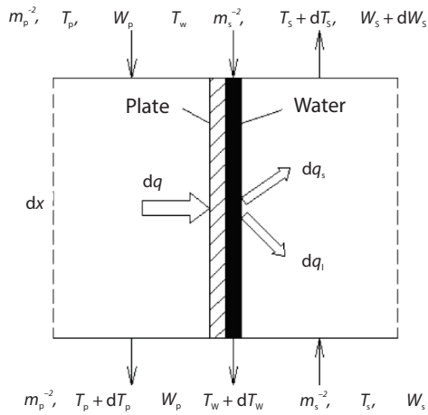
Figure 2. Cell control element applied for calculation
