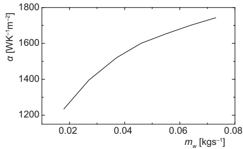
Figure 4. Effect of water mass flow rate on heat transfer coefficient ( T_e = 283\text{ K} )
