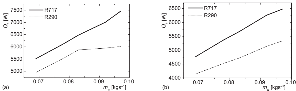
Figure 6. Effect of water mass flow rate on heat capacity of micro-fin evaporator ( T_e = 283\text{ K} ); (a) diameter of inner tube is 9.52 mm; (b) diameter of inner tube is 7.00 mm
