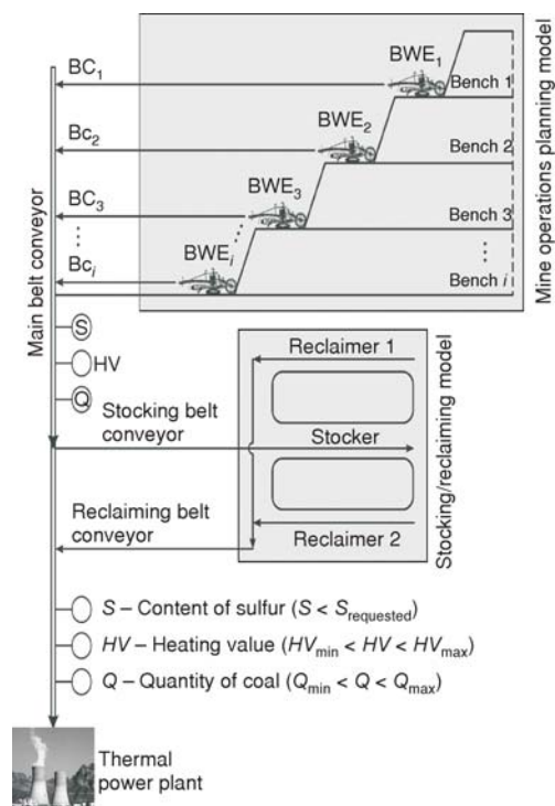
Figure 5. Technological scheme of coal homogenization in Kolubara surface mine
