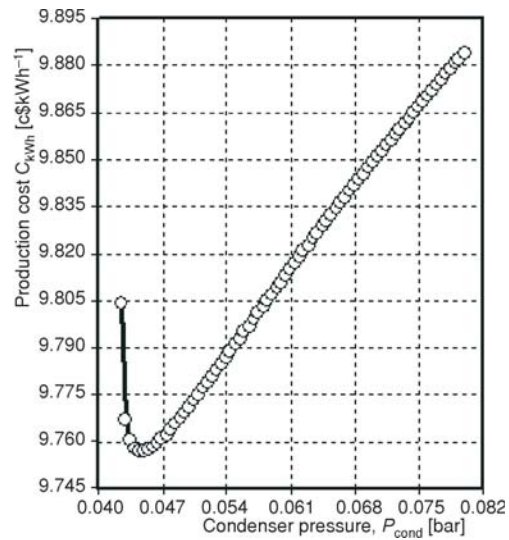
Figure 10. Effect of P_{\text{cond}} variations on production cost of the electricity
