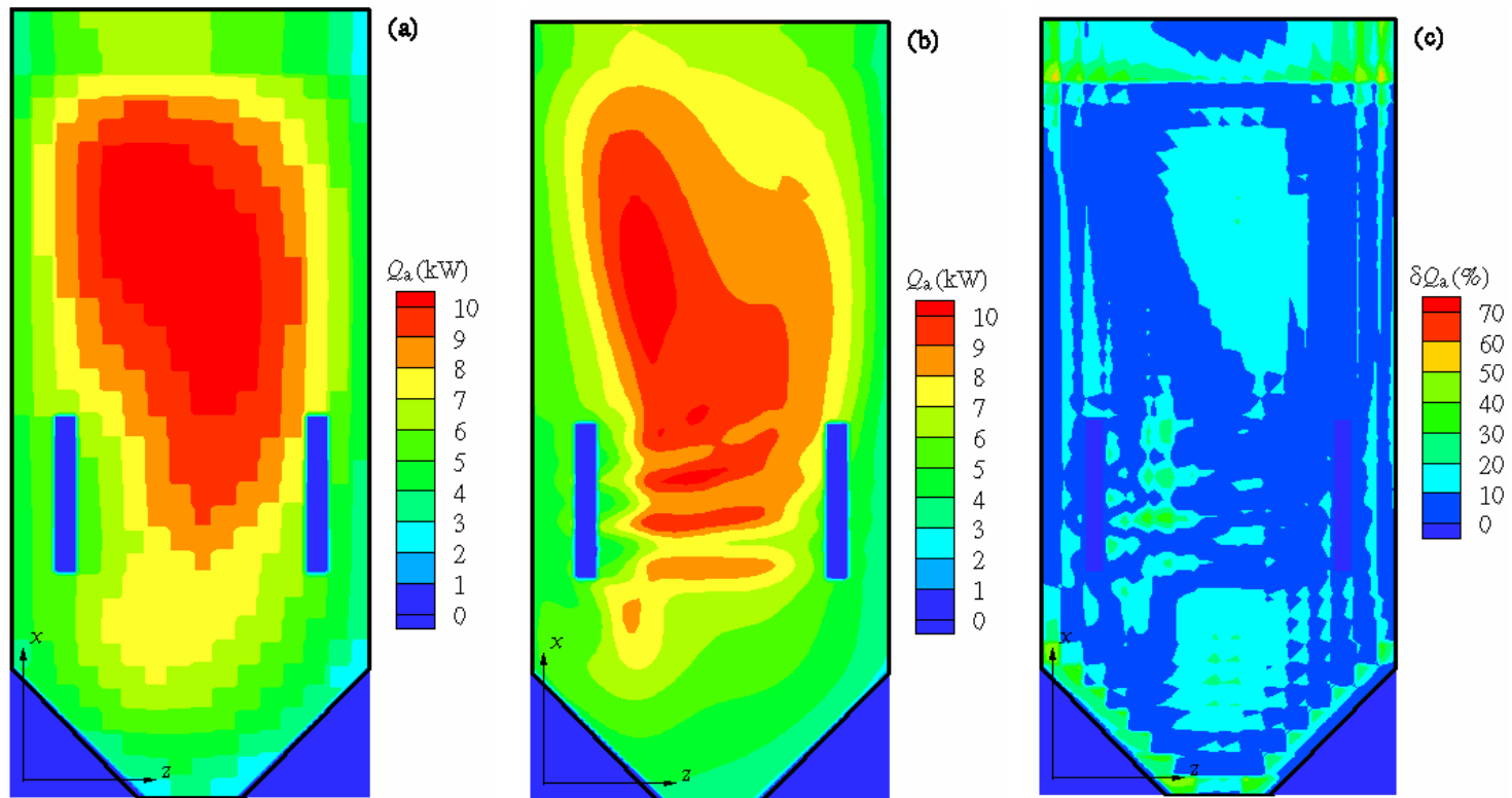
Figure 3. Absorbed radiative heat rate of rear furnace wall: (a) mathematical model containing HZM, (b) mathematical model containing SFM, (c) local difference
