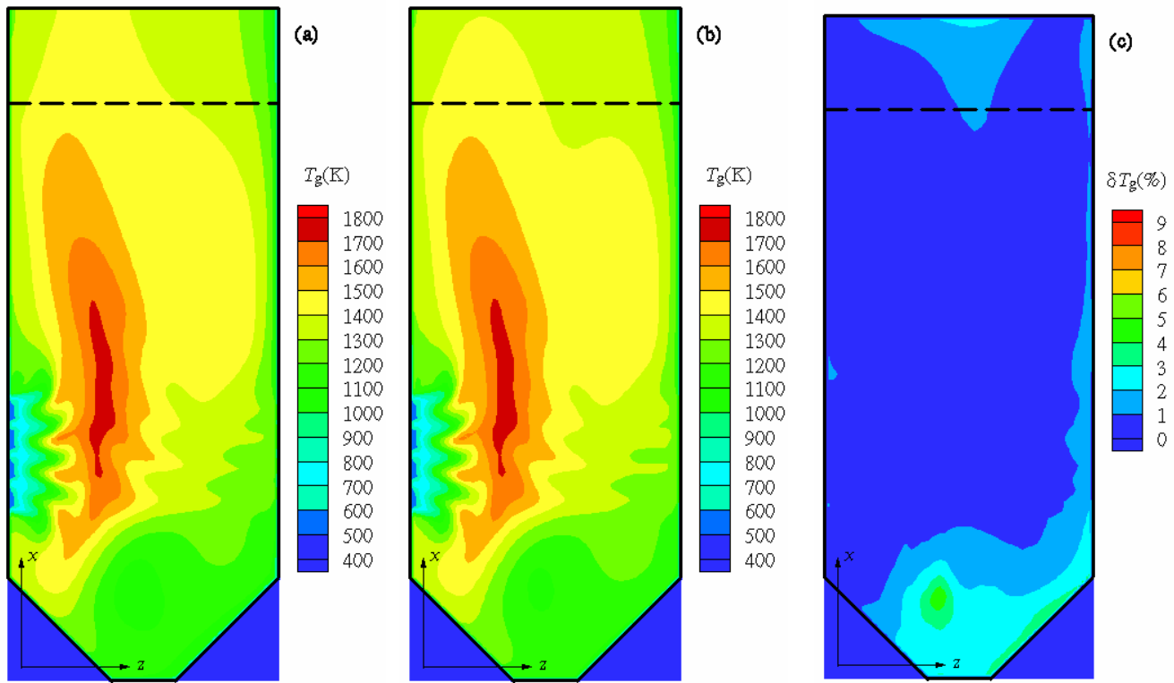
Figure 1. Gas-phase temperature at middle plane y = \text{const.} : (a) mathematical model containing HZM, (b) mathematical model containing SFM, (c) local difference
