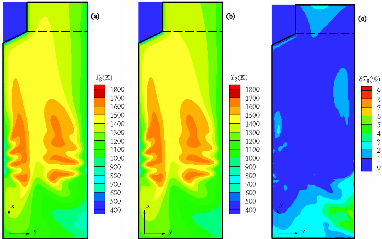
Figure 2. Gas-phase temperature at middle plane z = \text{const.} : (a) mathematical model containing HZM, (b) mathematical model containing SFM, (c) local difference
