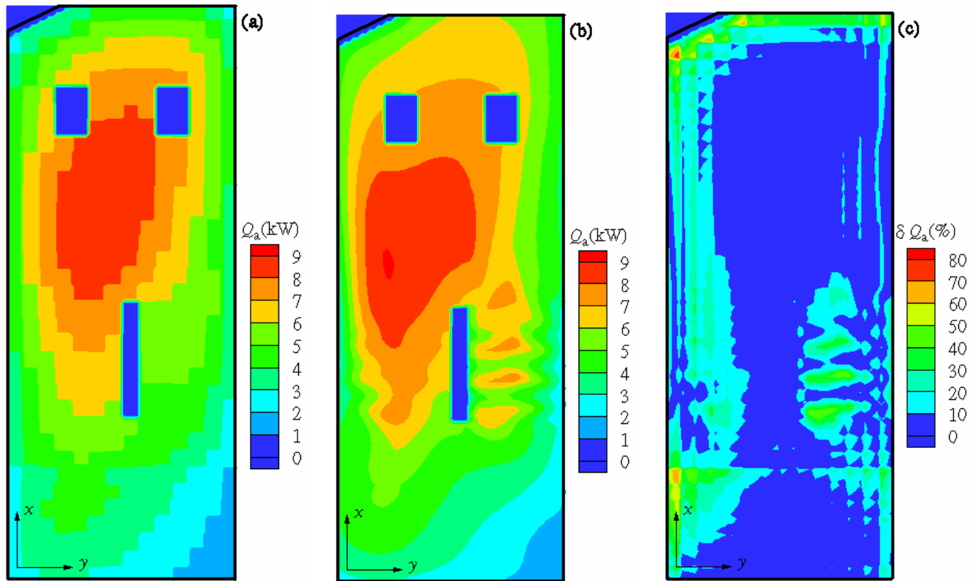
Figure 4. Absorbed radiative heat rate of right furnace wall: (a) mathematical model containing HZM, (b) mathematical model containing SFM, (c) local difference
