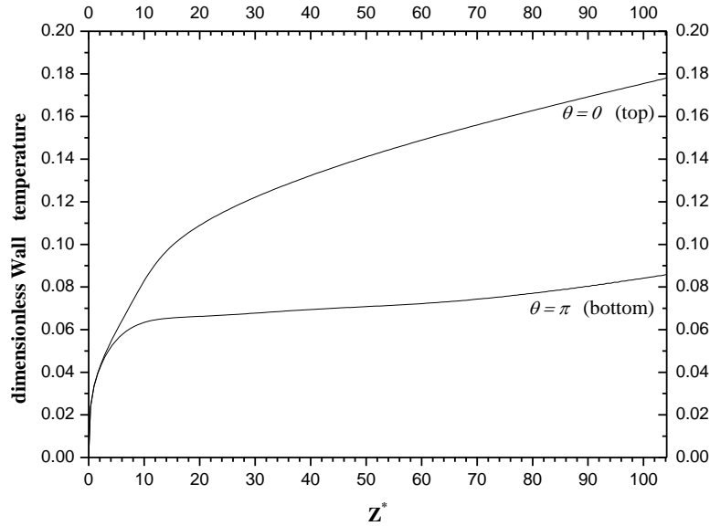
Figure 7. Axial variation of the outer wall temperature for Gr = 10^7 at the top and the bottom of the duct
