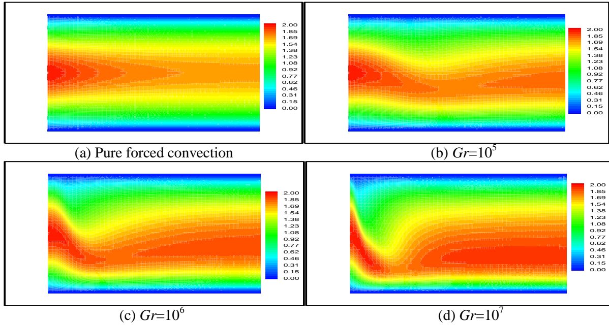
Figure 4. Development of the axial velocity
