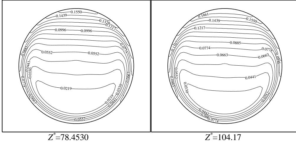
Figure 6. The isotherms distribution at the selected axial positions for Gr=10^6
