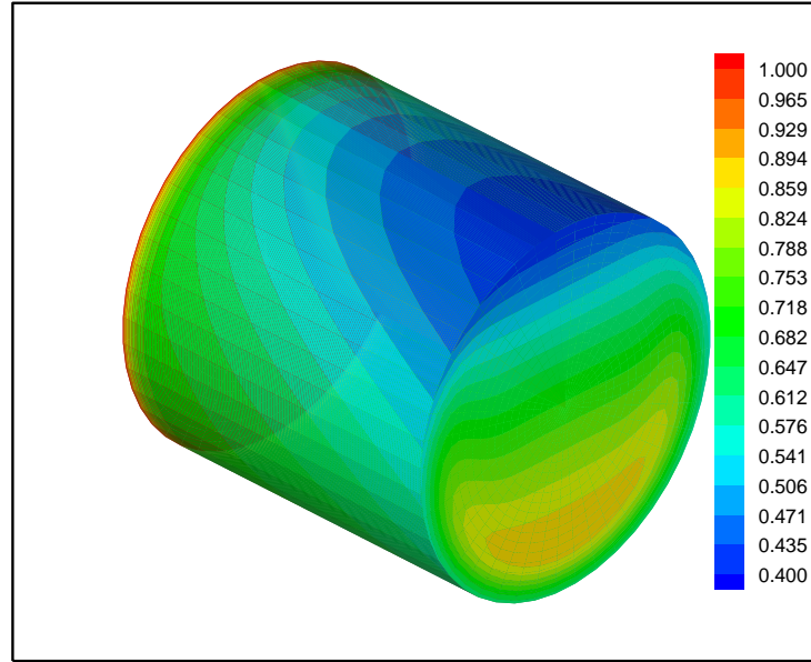
Figure 8. The dimensionless dynamic viscosity variation for Gr=5 \cdot 10^5
