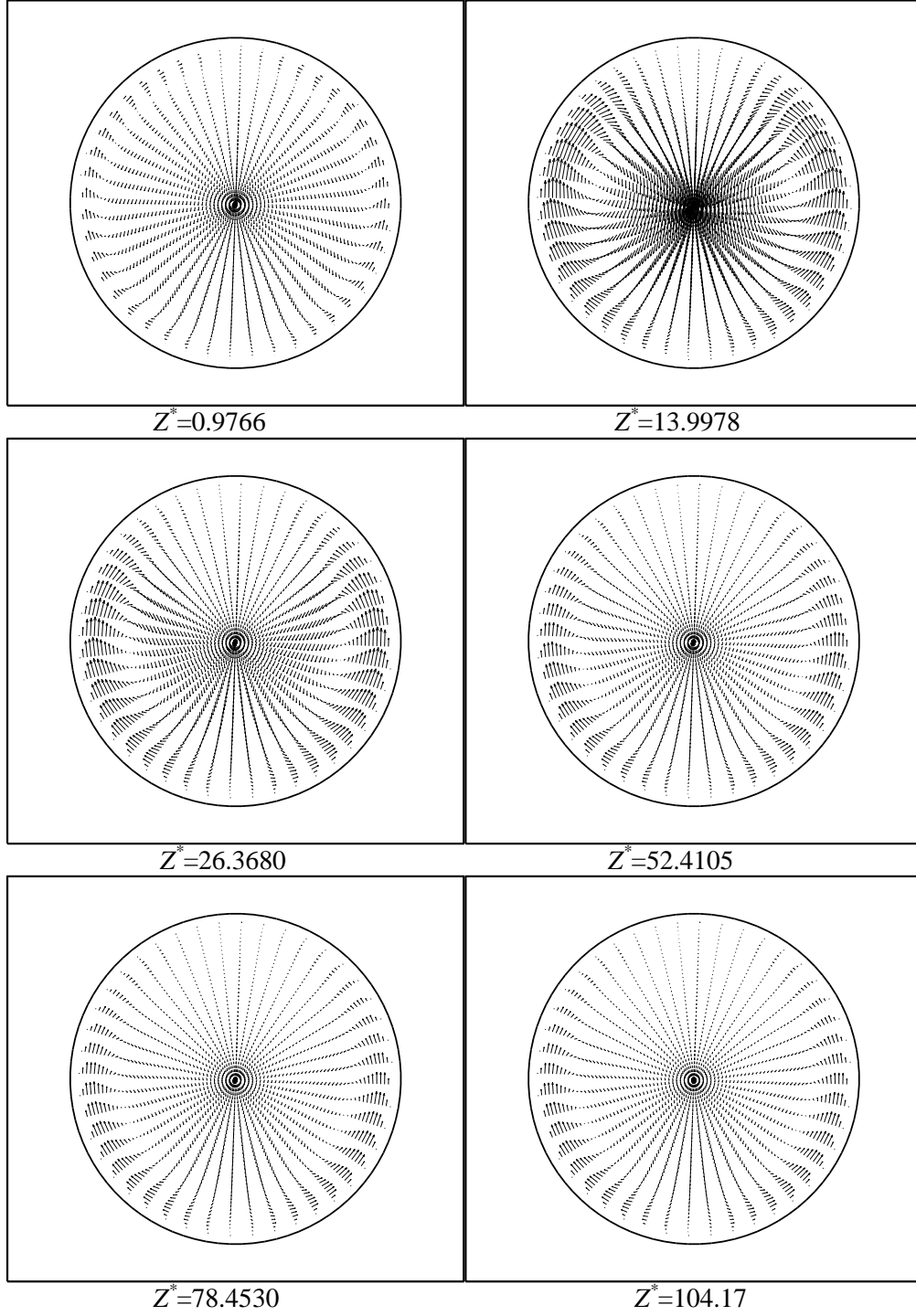
Figure 3. Development of the secondary flow at selected axial positions for Gr=10^6
