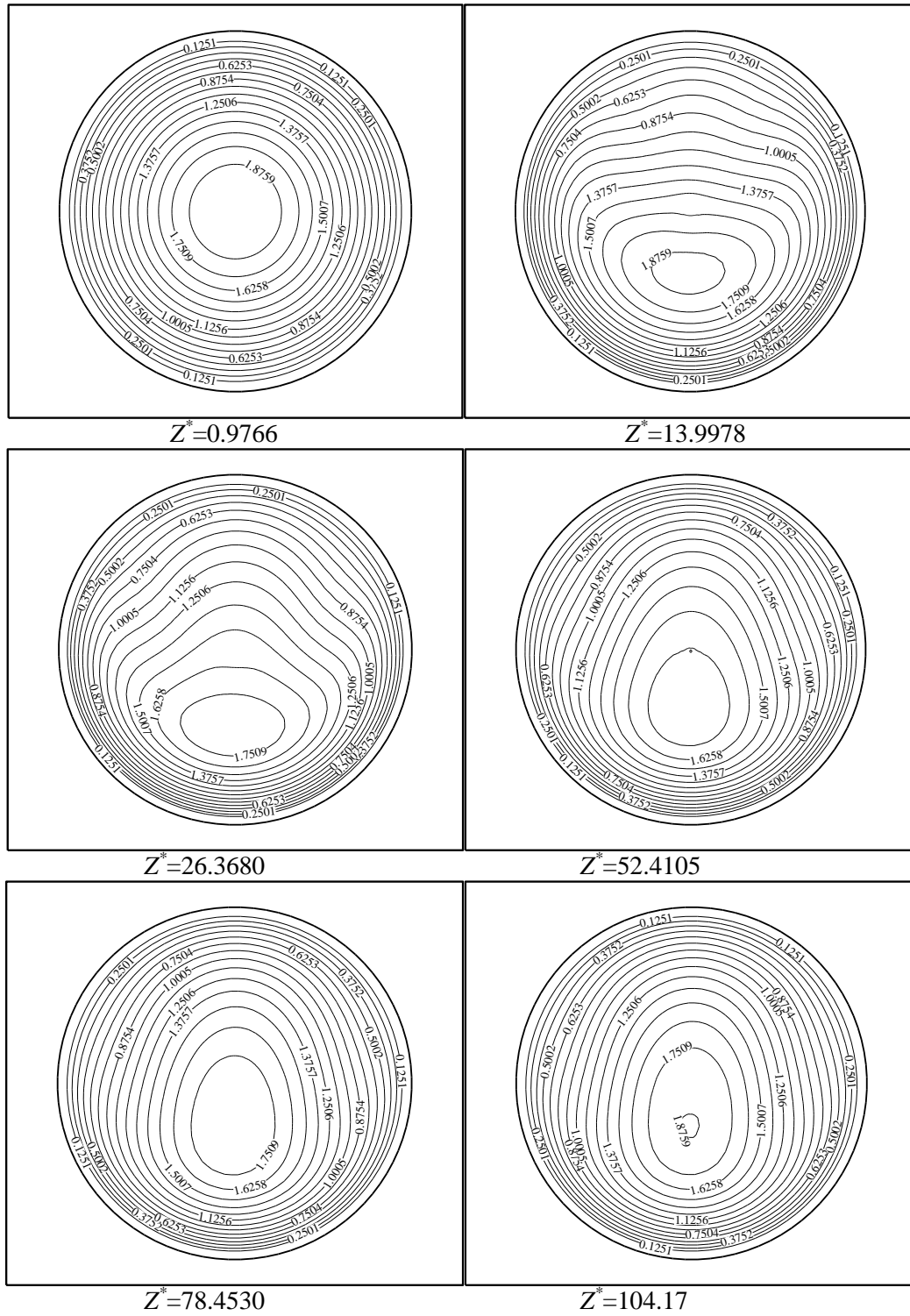
Figure 5. Axial velocity profiles at the selected pipe sections for Gr = 10^6 .
