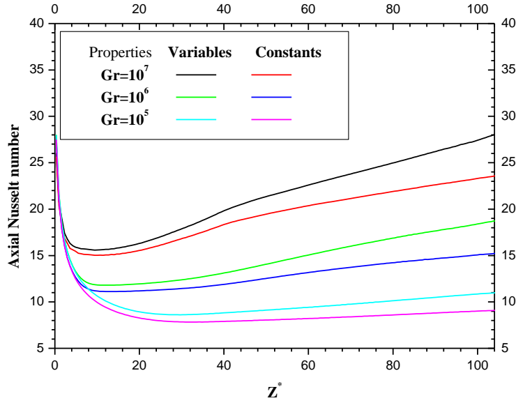
Figure 9. Comparison of axial Nusselt number between variables and constants fluid properties
