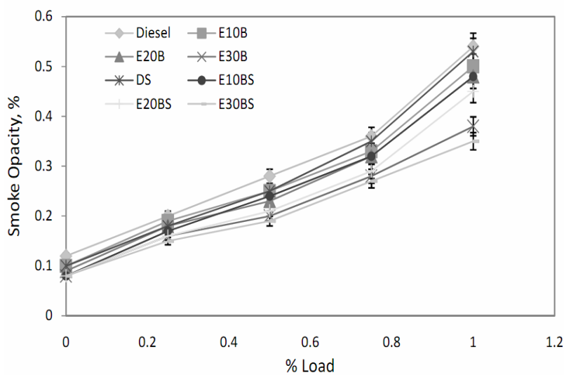
Figure 10. Variation of Smoke Opacity with load for ethanol diesel blends
