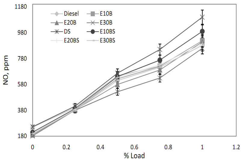
Figure 6. Nitric oxide emissions versus load for ethanol diesel blends
