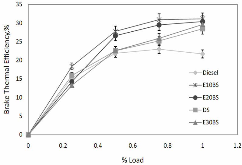
Figure 5. Brake thermal efficiency versus load for ethanol diesel blends with supercharging
