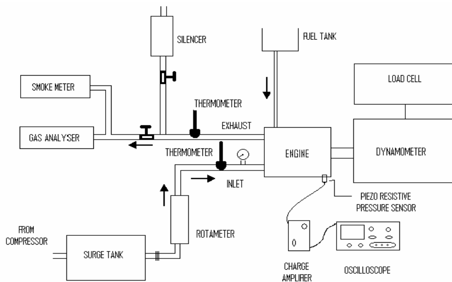
Figure 1: Schematic of engine test setup
