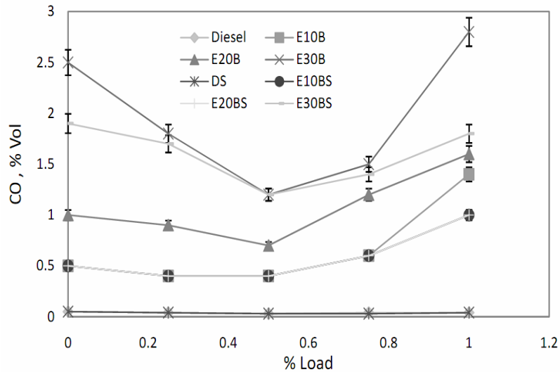
Figure 7. Carbon monoxide emissions versus load for ethanol diesel blends
