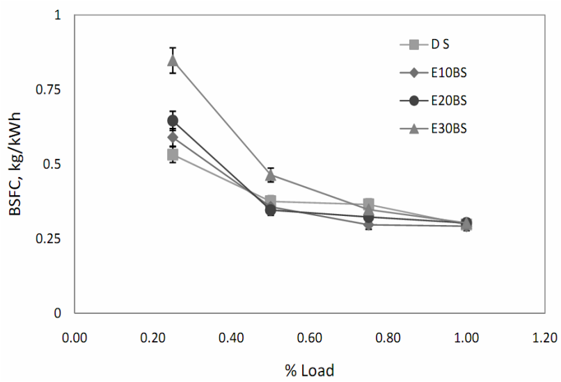
Figure 3. Variation of BSFC with load for ethanol diesel blends with supercharging
