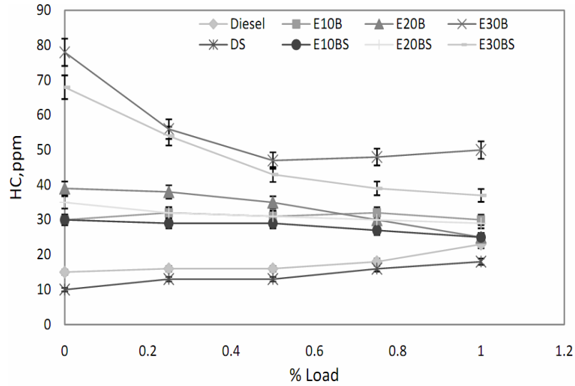
Figure 8. Variation of hydrocarbon emissions versus load for ethanol diesel blends
