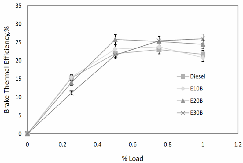
Figure 4. Brake thermal efficiency versus load for ethanol diesel blends
