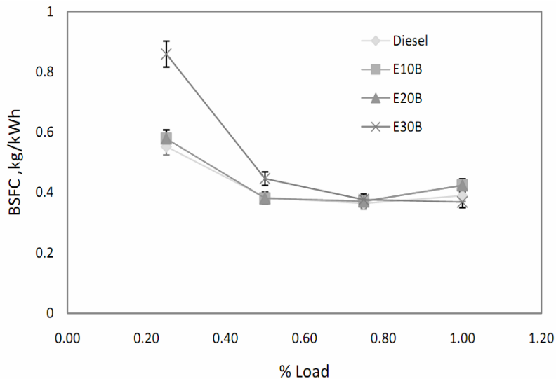
Figure 2. Variation of brake specific fuel consumption with load for ethanol diesel blends
