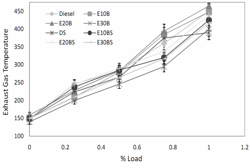
Figure 9. Variation of exhaust gas temperature with load for ethanol diesel blends
