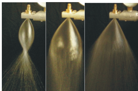
Figure 16. Spray formation stages with regard to fluid swirl
