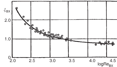
Figure 2. Diagram of the amount of input channel resistance \xi_{BX} and Reynolds number [1]
