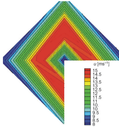
Figure 24. Velocity distribution of spray in a normal plan (color image see on our web site)
