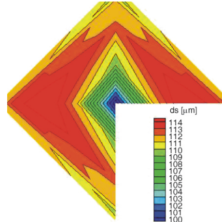
Figure 25. SMD distribution of spray in a normal plan (color image see on our web site)
