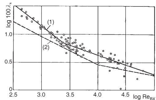
Figure 4. Relationship between value of friction and the input Reynolds number [1] (1) experimental relation, (2) theoretical relations
