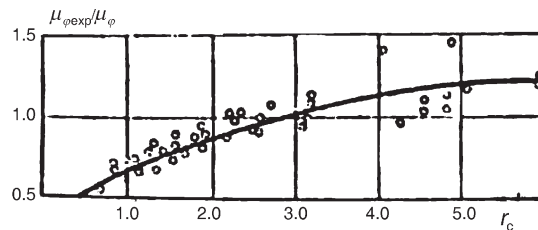
Figure 8. Correction factor of coefficient flow vs. swirl radius
