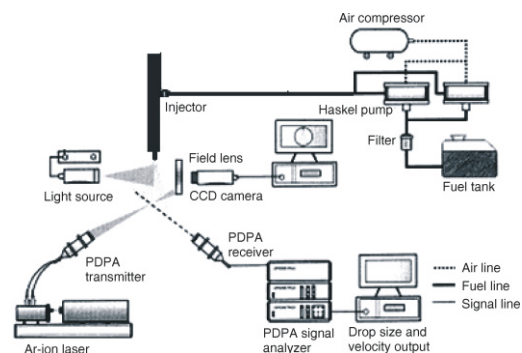
Figure 22. Phase Doppler analysis system
