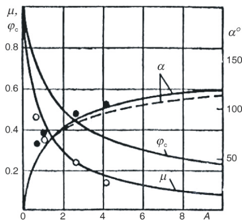
Figure 6. Relationship of discharge coefficient and nozzle contraction coefficient and spray angle to the geometric characteristic of injector [2]
