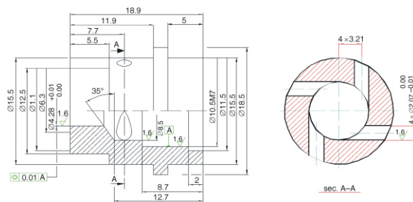
Figure. 10 Manufacturing diagram external nozzle
