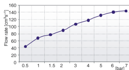
Figure 15. Flow rate of external nozzle vs. pressure
