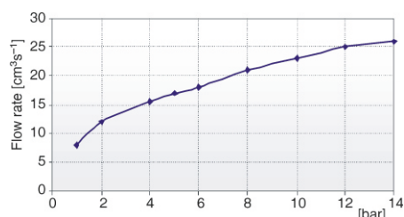
Figure 14. Flow rate of internal nozzle vs. pressure
