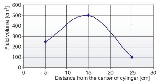
Figure 21. Spray distribution of the injector in each cylinder
