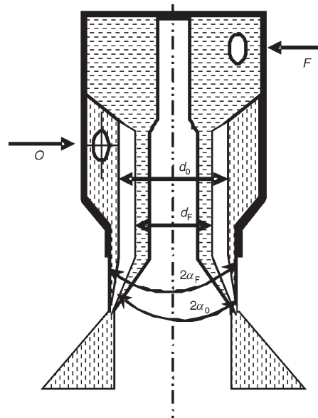
Figure 7. Double-base external mixing injector [2]
