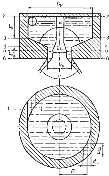
Figure 1. Double base-swirl injector cross-section [1]
