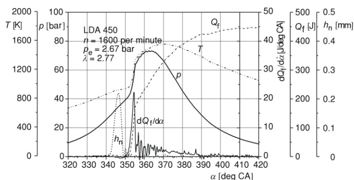
Figure 13. The results of pressure trace analysis: rate of heat release dQ_f/d\alpha , cumulative heat released Q_f , and mean gas temperature T ; h_n injector needle lift
