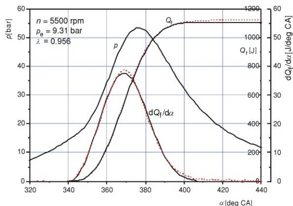
Figure 6. The comparison of modeled rate of heat release (solid line) and the rate of heat released obtained by the analysis of modeled pressure diagram using the described model (dashed line)
