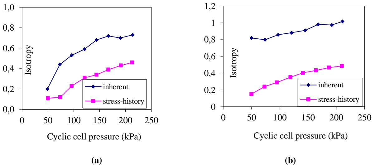
Figure 3. (a) Sand&gravel and (b) limestone anisotropy test results [14].
