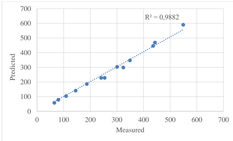
Figure 7. Axial strain predictions for limestone.
