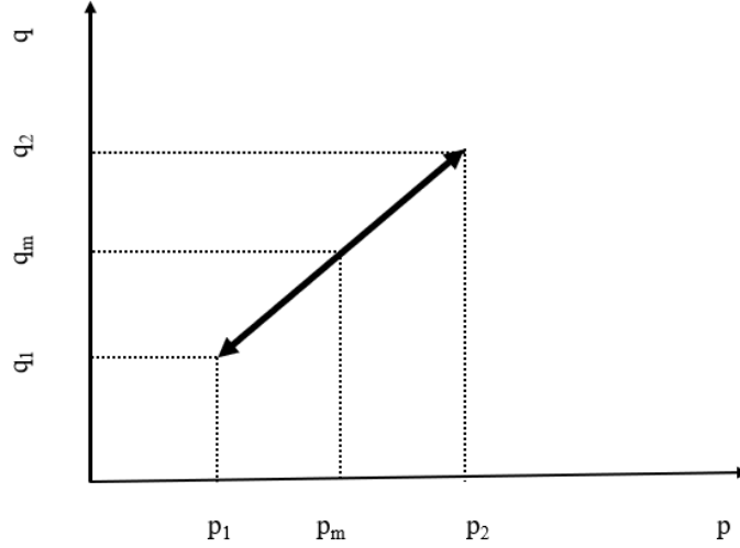
Figure 4. Stress paths in p-q space.
