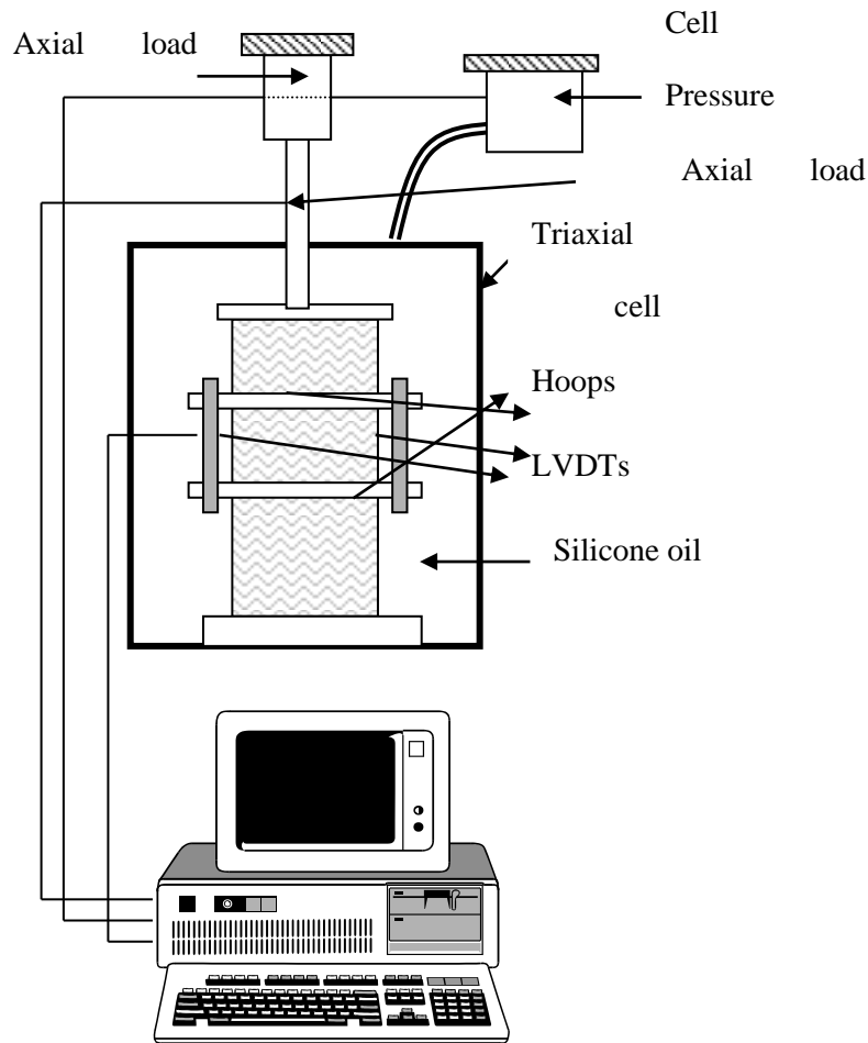
Figure 2. Repeated load triaxial equipment [14].
