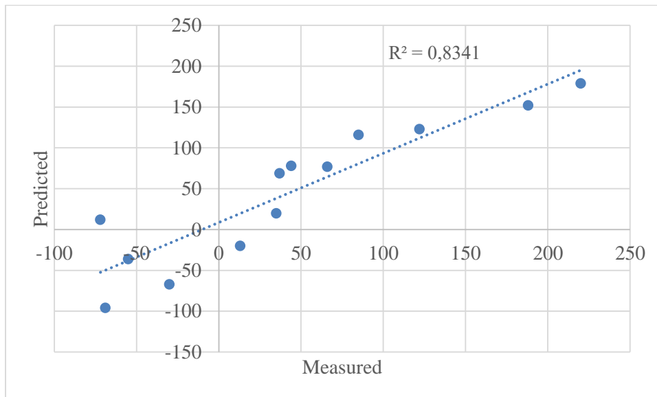
Figure 8. Radial strain predictions for limestone.
