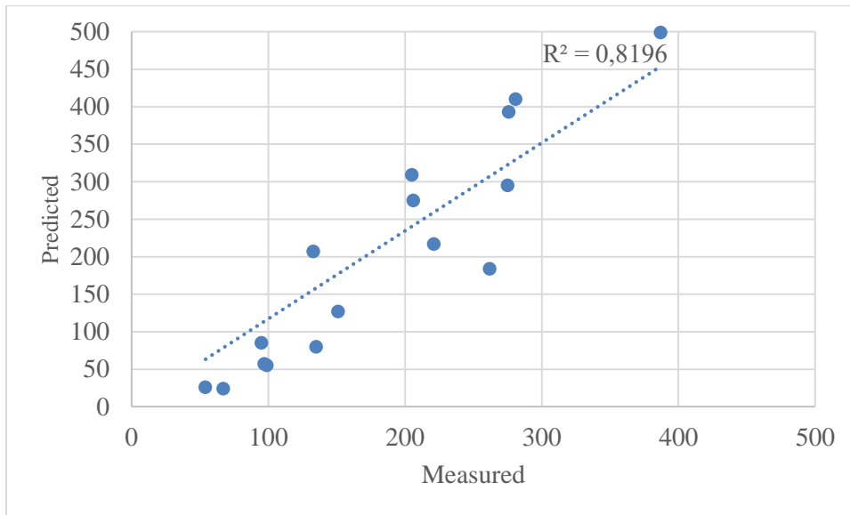
Figure 5. Axial strain predictions for sand&gravel.
