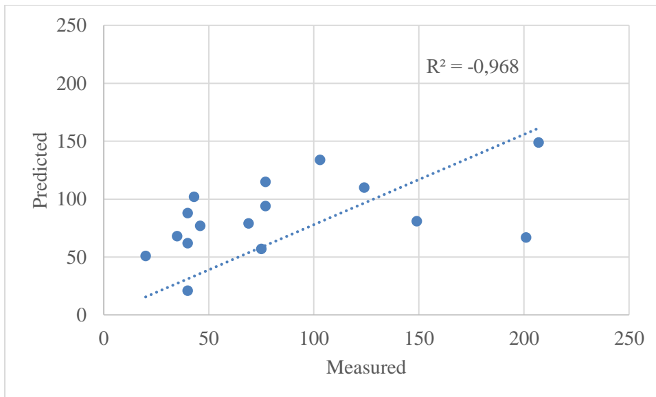
Figure 6. Radial strain predictions for sand&gravel.
