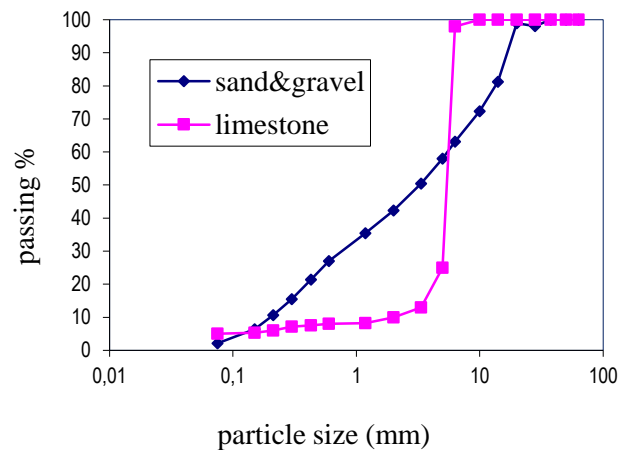
Figure 1. Grading curves for sand&gravel and limestone [14].
