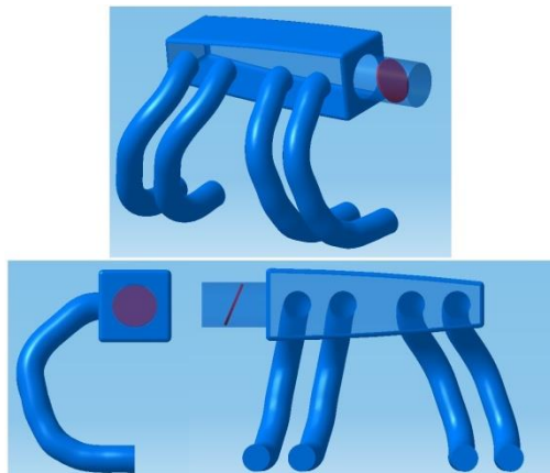
Figure 2. 3D model of the intake manifold
