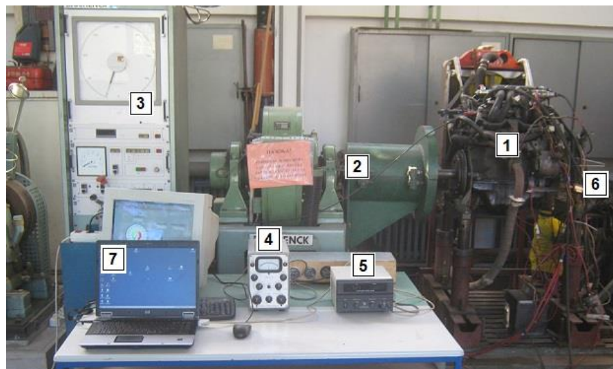
Figure 6. Experimental setup [8]
