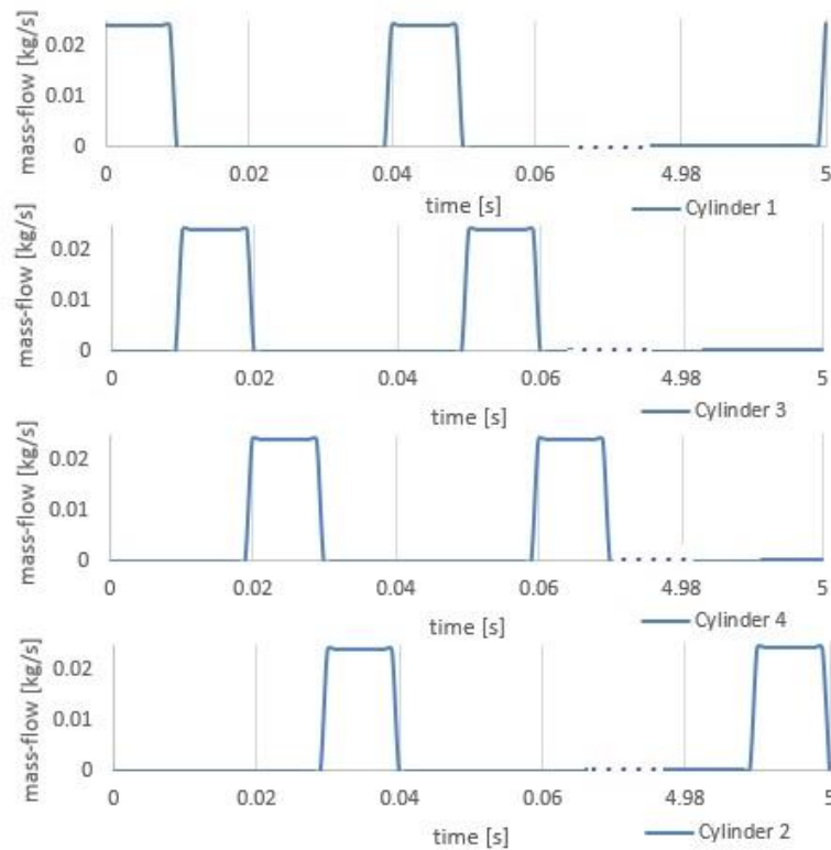
Figure 5. Periodical function of intake processes
