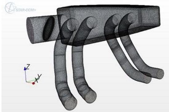
Figure 3. Mesh CFD model of the intake manifold
