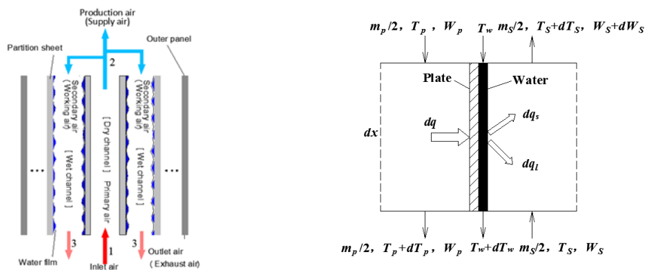
Figure 1. Schematic of counter flow HMX Figure 2. cell control element applied for calculation
