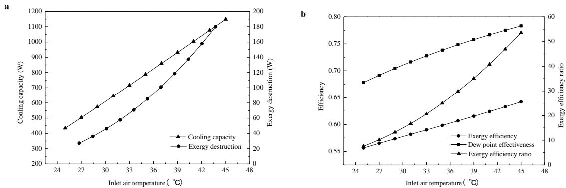
Figure 4. Influence of inlet air temperature: (a) cooling capacity and exergy destruction (b) exergy efficiency, dew point effectiveness and exergy efficiency ratio
