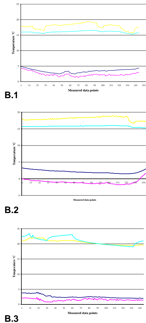
Figure 5. The inside and outside air and surface wall temperature measured in situ
