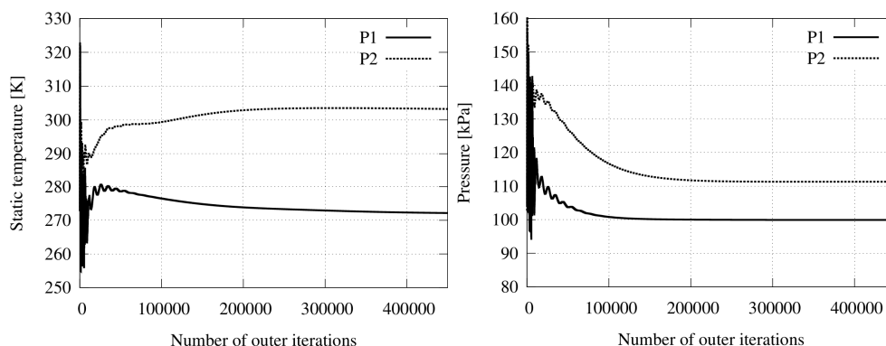
Figure 3. Changes of temperature and pressure during iteration procedure. Solver steadyCompressibleTEFoam, mesh M2, k - \varepsilon turbulence model. Point coordinates: P1(0.01,0.001,0), P2(0.3,0.001,0).
