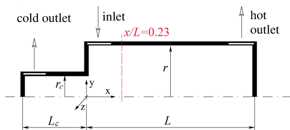
Figure 1. Geometry of the vortex tube, [16].
