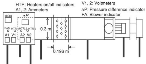
Figure 2. Experimental set-up (front view)
