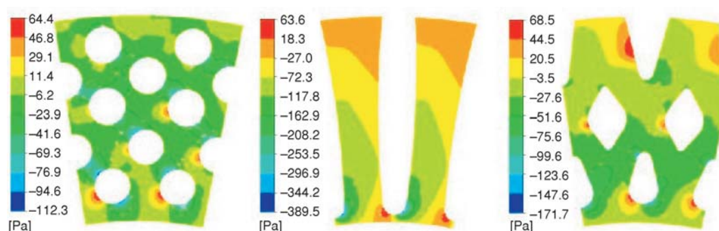
Figure 11. Pressure distribution on mid plane for CP, MTRV, and DP at 1000 rpm (for color image see journal web site)
